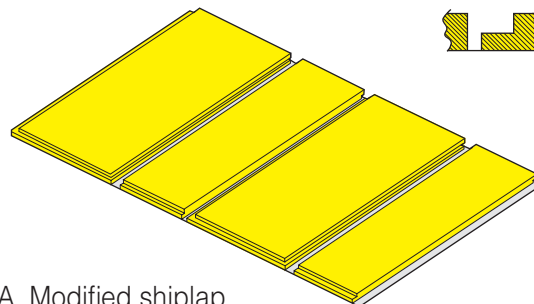
Fig. 2-3A. Modified shiplap
