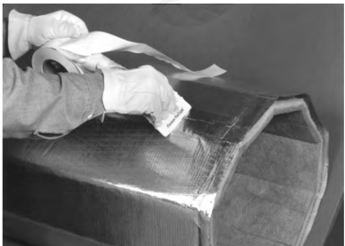
Fig. 3-34C. Taping longitudinal joint of ten sided duct.
