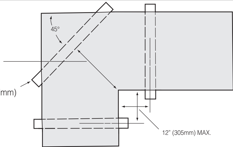
Fig. 6-5A. Elbow support.
