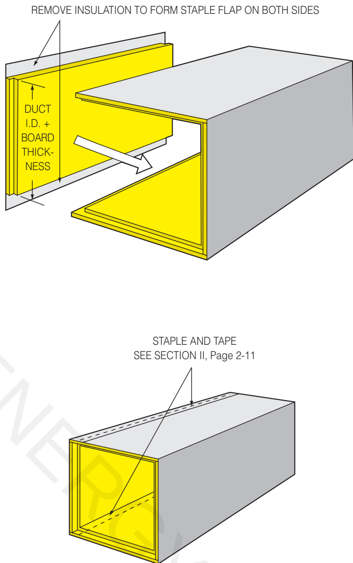
Fig. 7-5. Replacing square edge panel.
