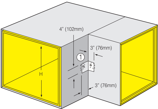
Fig. 5-15A. Sheet metal angle reinforcement at throat, 90° elbow.
