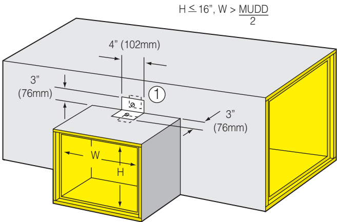
Fig. 5-16A. Sheet metal angle reinforcement, top of branch.
