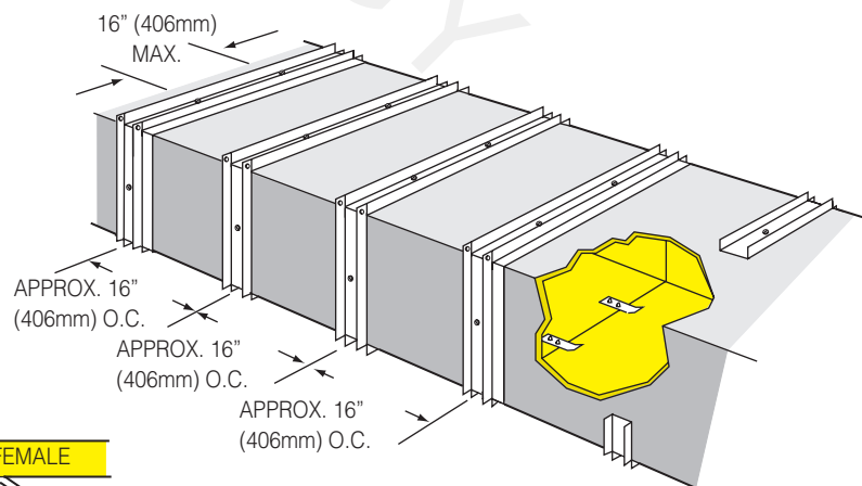
Fig. 5-12C. Channel reinforcement, 16" (406mm) (approx.) centers, 48" (1219mm) duct modules.
