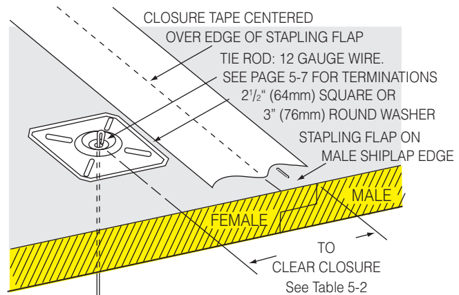
Fig. 5-4A. Tie rod reinforcement.
