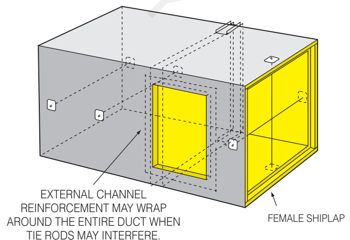
Fig. 5-23C. Channel reinforcement. See Page 5-13.
