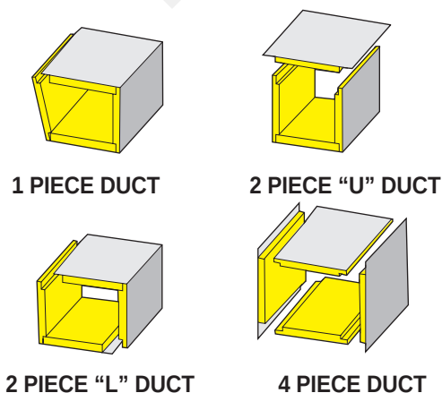
Fig. 2-4. Four ways to make a duct section.
