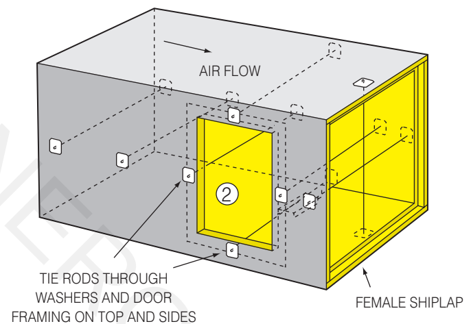
Fig. 5-23B. Reinforcement of access door framing.
