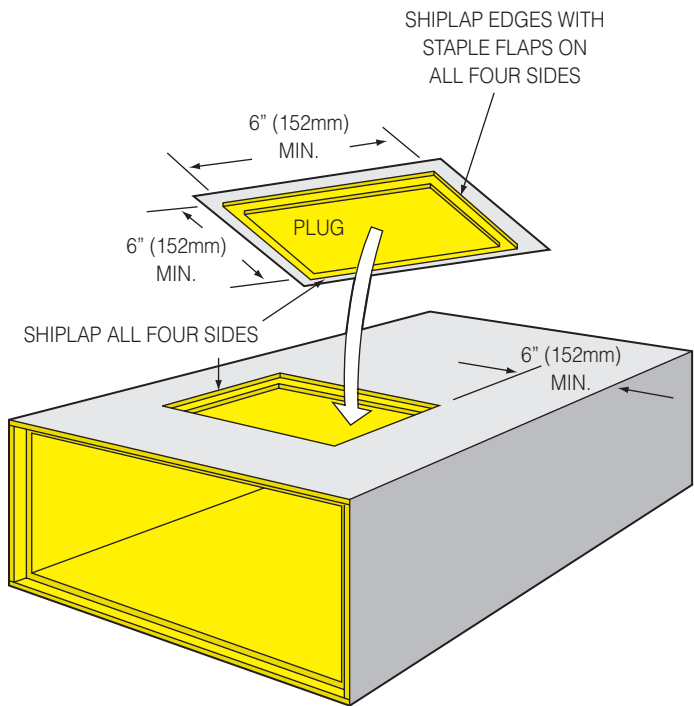
Fig. 7-3A. Repairing major damage to one panel.
