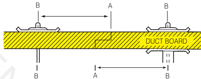
Fig. 5-4A. Tie rod reinforcement.
