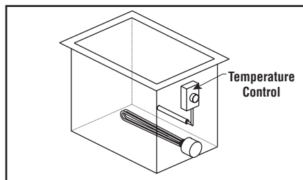
MT — screwed into tank wall parallel to bottom for use as a hot water rinse.
