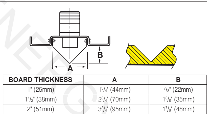
Fig. 2-5E. V-Groove Tool - Cuts 90° V-grooves for corner folds when modified shiplap grooving method is not used.
