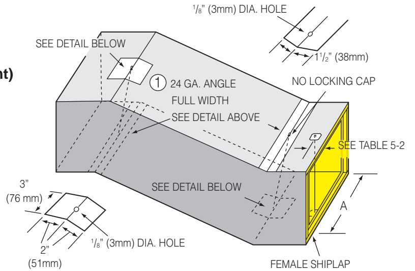
Fig. 5-21A. Offset reinforcement with sheet metal plates and tie rods.
