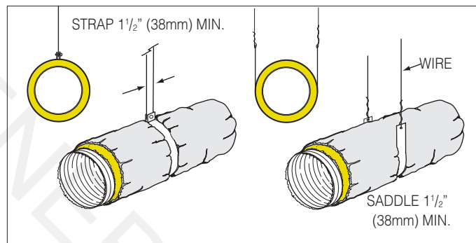
Fig. 6-9B. Hangers or saddle material must be at least 1 1/2" (38mm) wide to prevent restriction of the internal diameter of the flexible duct.
