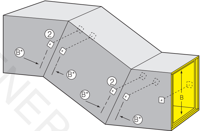
Fig. 5-20B. Offset reinforcement, cheek panels with butt joints.
