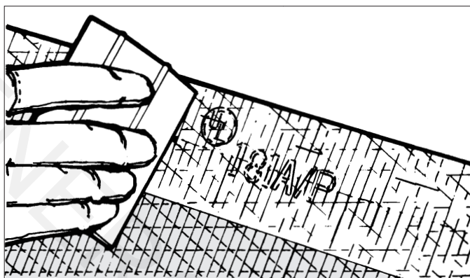
Fig. 4-3B. Rub tape firmly with plastic sealing tool until the facing reinforcement shows clearly through the tape. Avoid tearing or puncturing tape at staples.
