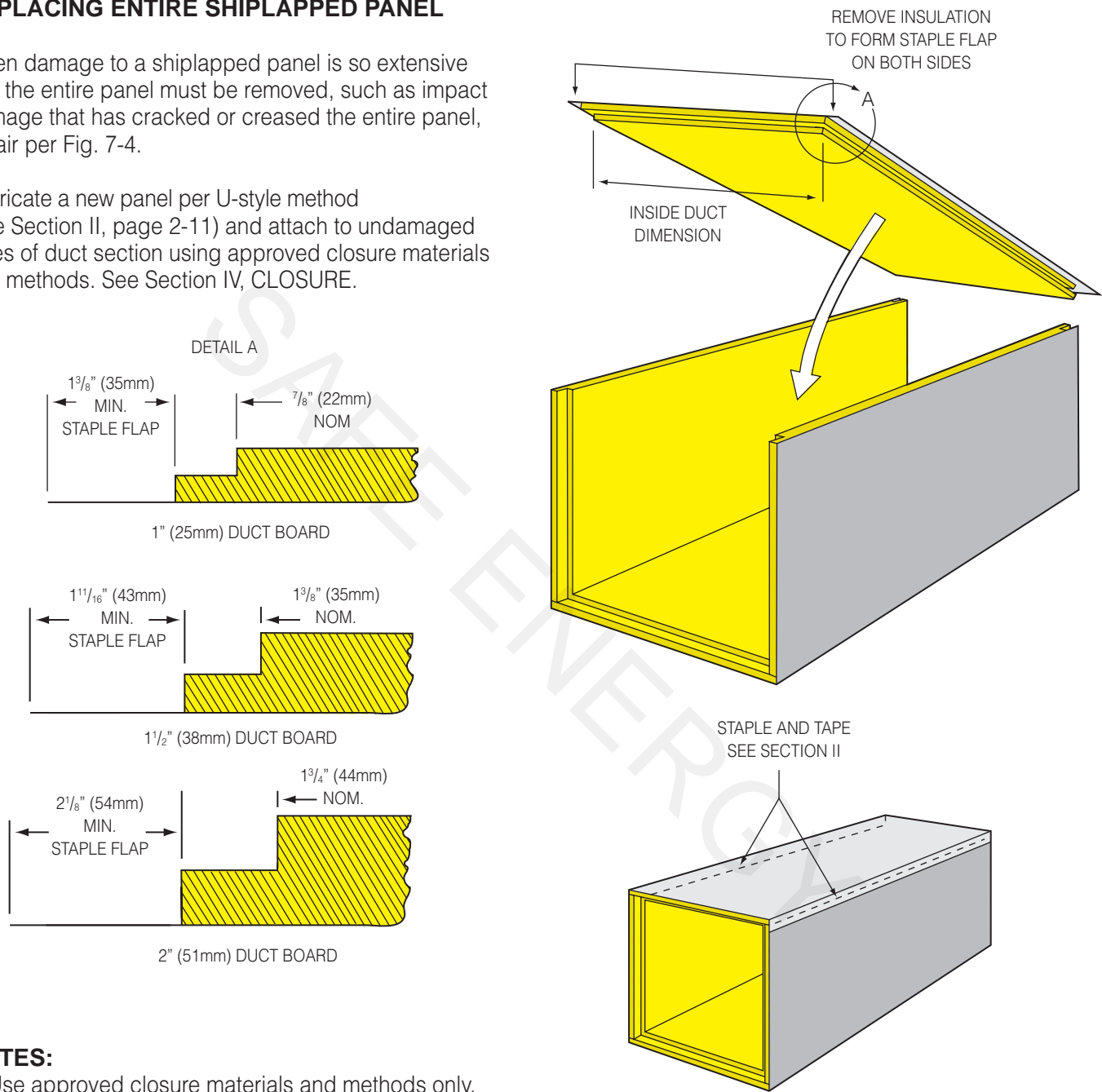
Fig. 7-4. Replacing shiplapped panel.
