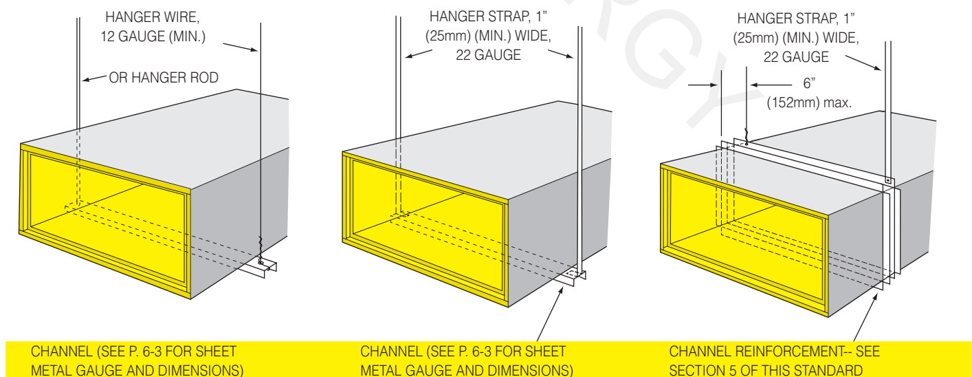
Fig. 6-2. Approved hanger configurations for rectangular fibrous glass ducts.
