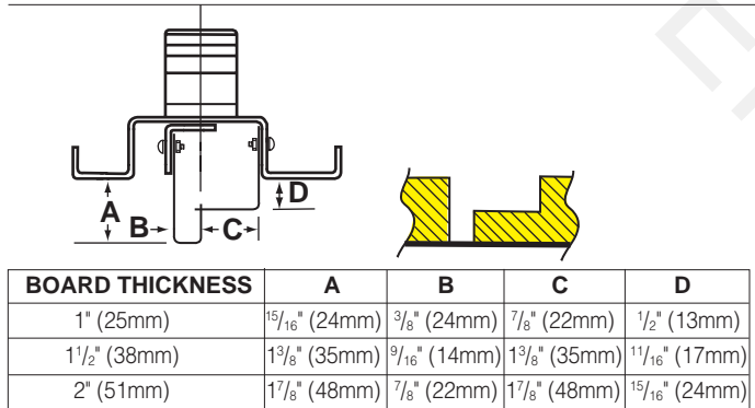
Fig. 2-5B. Modified Shiplap Tool - Removes insulation for shiplap corner folds. Reversing the tool allows both left hand and right hand shiplaps to be cut.
