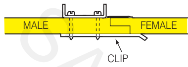
Fig. 5-12A. Channel reinforcement, 48" (1219mm) (approx.) centers, 48" (1219mm) duct modules.
