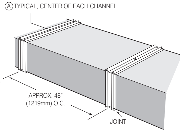
Fig. 5-10A. Channel reinforcement, approx. 48" (1219mm) on centers, 48" (1219mm) duct modules.
