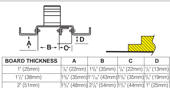
Fig. 2-5F. Shiplap and End Cut-Off Tool - Cuts shiplap on end of board for longitudinal corner closure, plus staple flap. May also be used in some fitting fabrication techniques.
