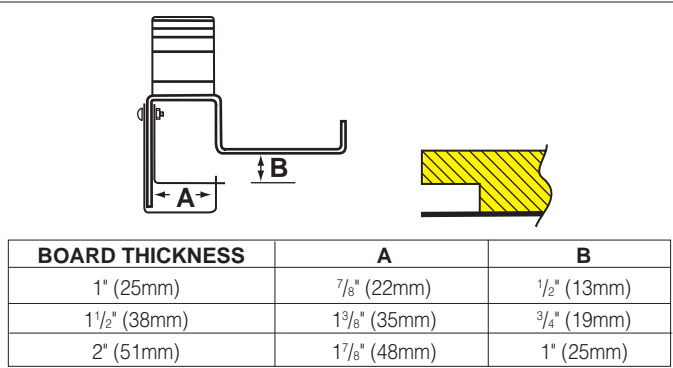
Fig. 2-5D. Male Shiplap Tool - Cuts male slip joint which mates with female slip joint to connect two duct sections.
