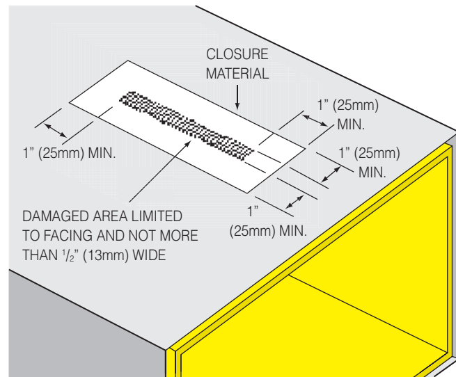
Fig. 7-2A. Repair of minor facing damage - less than 1/2" (13mm) wide.
