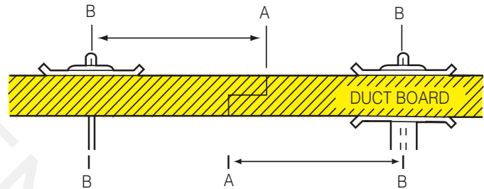
Fig. 5-4A. Tie rod reinforcement.
