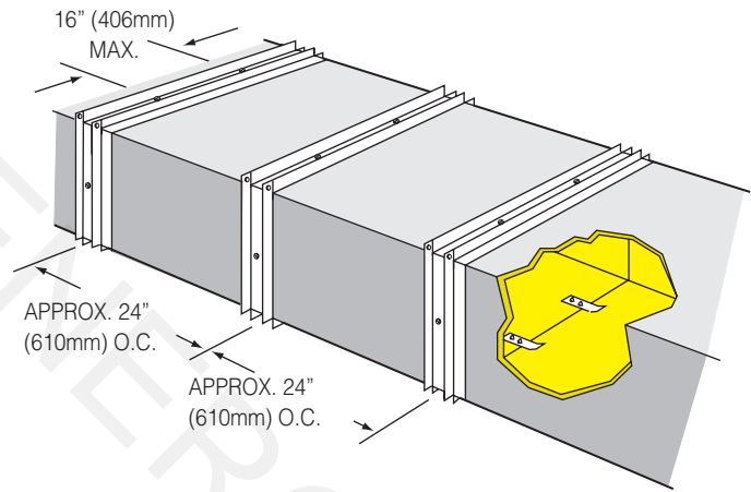
Fig. 5-12B. Channel reinforcement, 24" (610mm) (approx.) centers, 48" (1219mm) duct modules.
