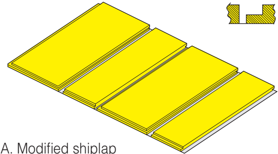
Fig. 2-3A. Modified shiplap
