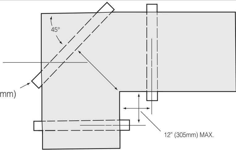
Fig. 6-5A. Elbow support.
