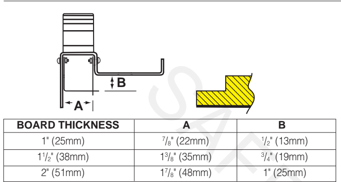
Fig. 2-5A. Female Shiplap Tool - Cuts female slip joint. Also cuts seating edge of duct board at longitudinal closure corner.
