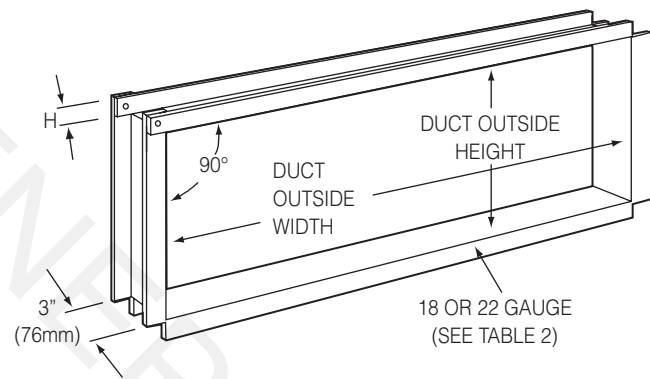
Fig.5-9B. Detail of channel reinforcement.
