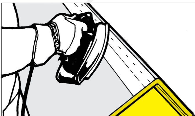
Fig. 4-3C. When applying pressure sensitive tape at temperatures below 50°F (10°C), use iron set at 400°F (204°C) to pre-heat area to be taped, then press tape in place.
