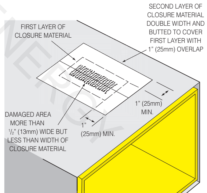
Fig. 7-2B. Repair of minor facing damage - 1/2" (13mm) wide or greater.
