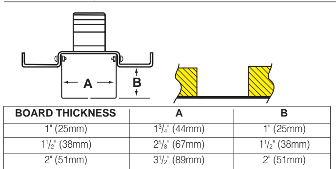
Fig. 2-5C. Staple Flap Tool - Used with straight knife to make staple flap and end cut
