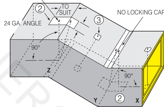
Fig. 5-21B. Offset reinforcement with tie rods through throat.
